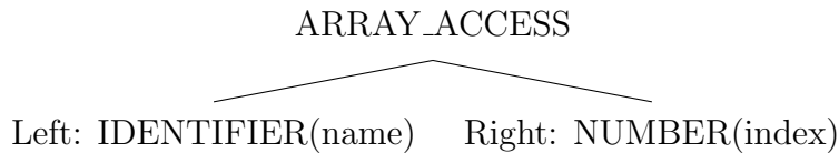
Figure 10: How array access is parsed
